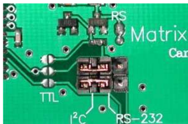
Figure 10: I 2 C
