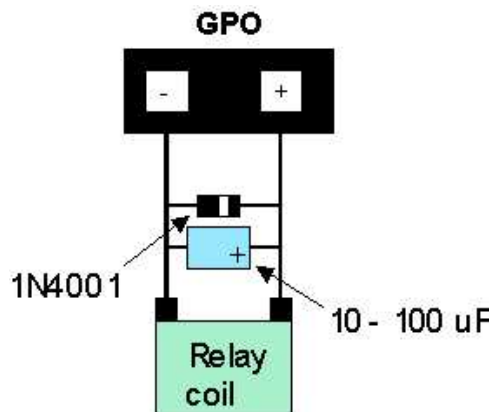
Figure 18: Clamping a Relay
