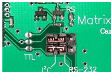
Figure 12: TTL Communications
