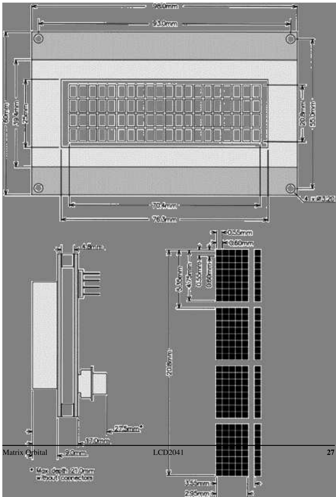
Figure 20: Physical Layout
